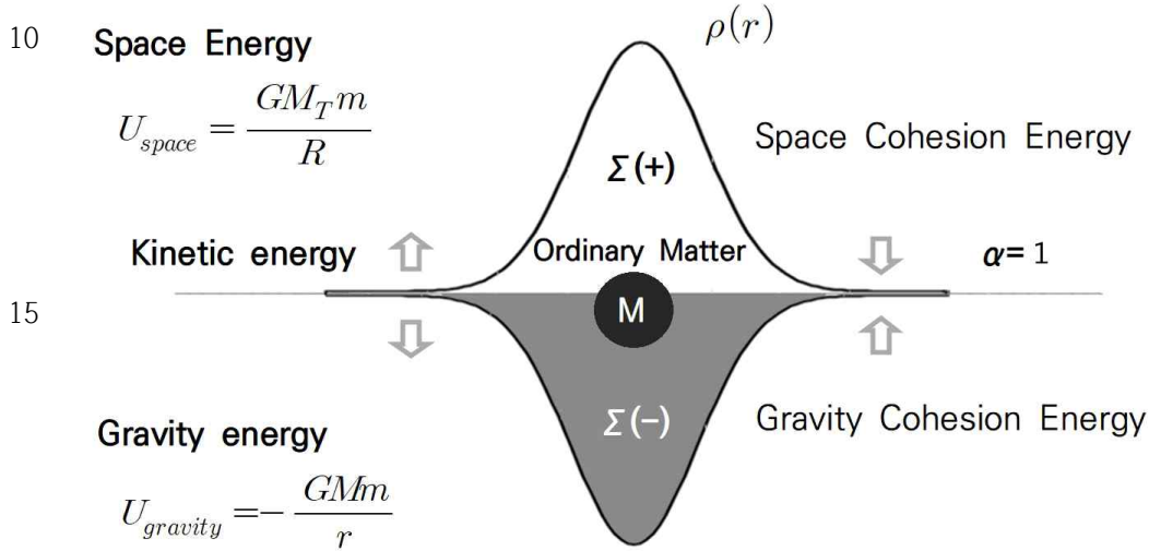
Figure 1. Space Equilibrium With Mass Energy Fields
